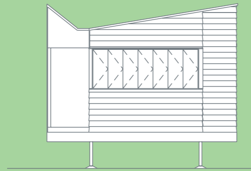
2 ELEVATION 5000 EXPANDER
