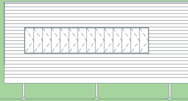
3 ELEVATION 8000 EXPANDER
