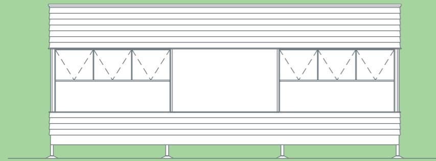
4 ELEVATION 9000 EXPANDER
