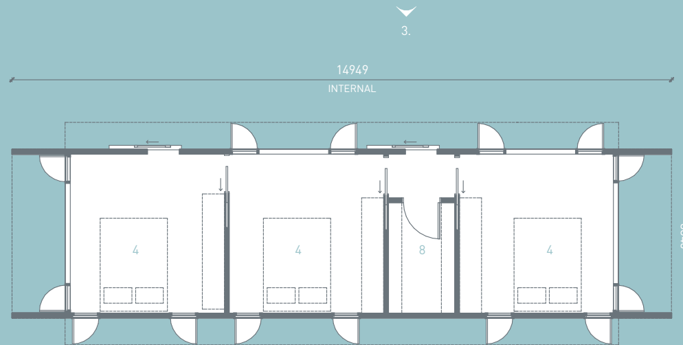
1 FLOOR PLAN 3B
